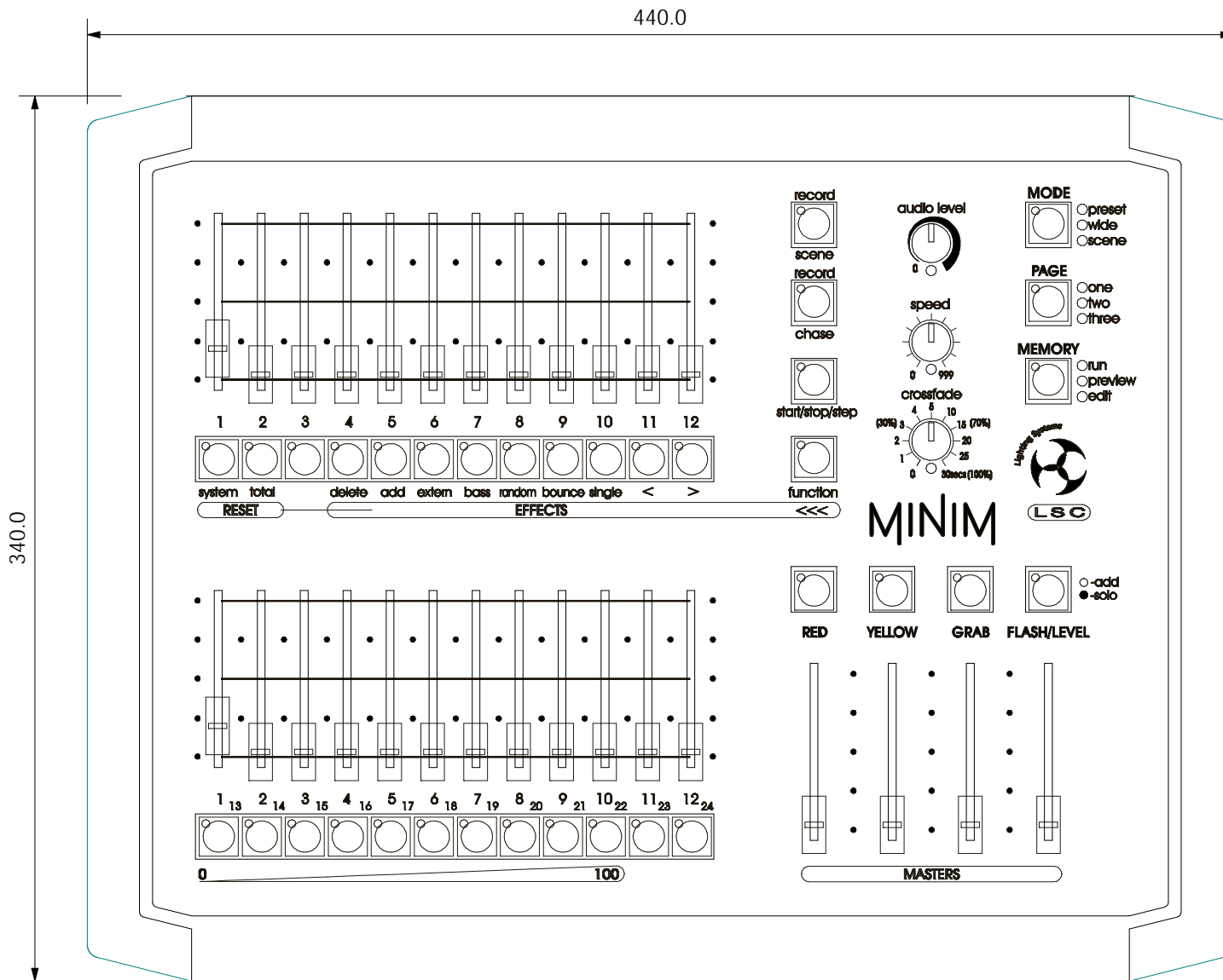
MINIM Console outline drawing LSC Lighting Systems
