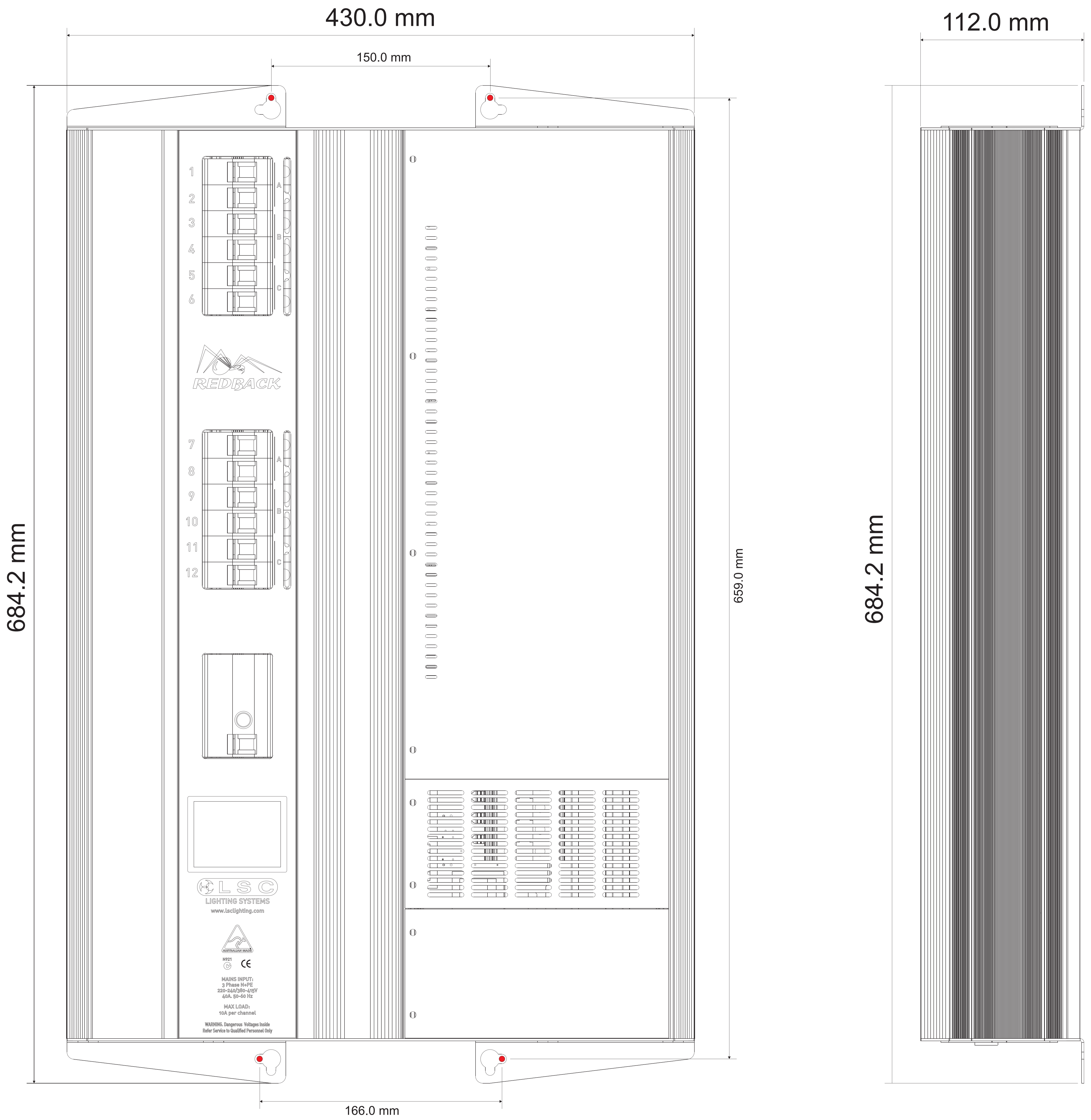
Redback 12 Channel Installation Dimmer Outline Drawing LSC Lighting systems
