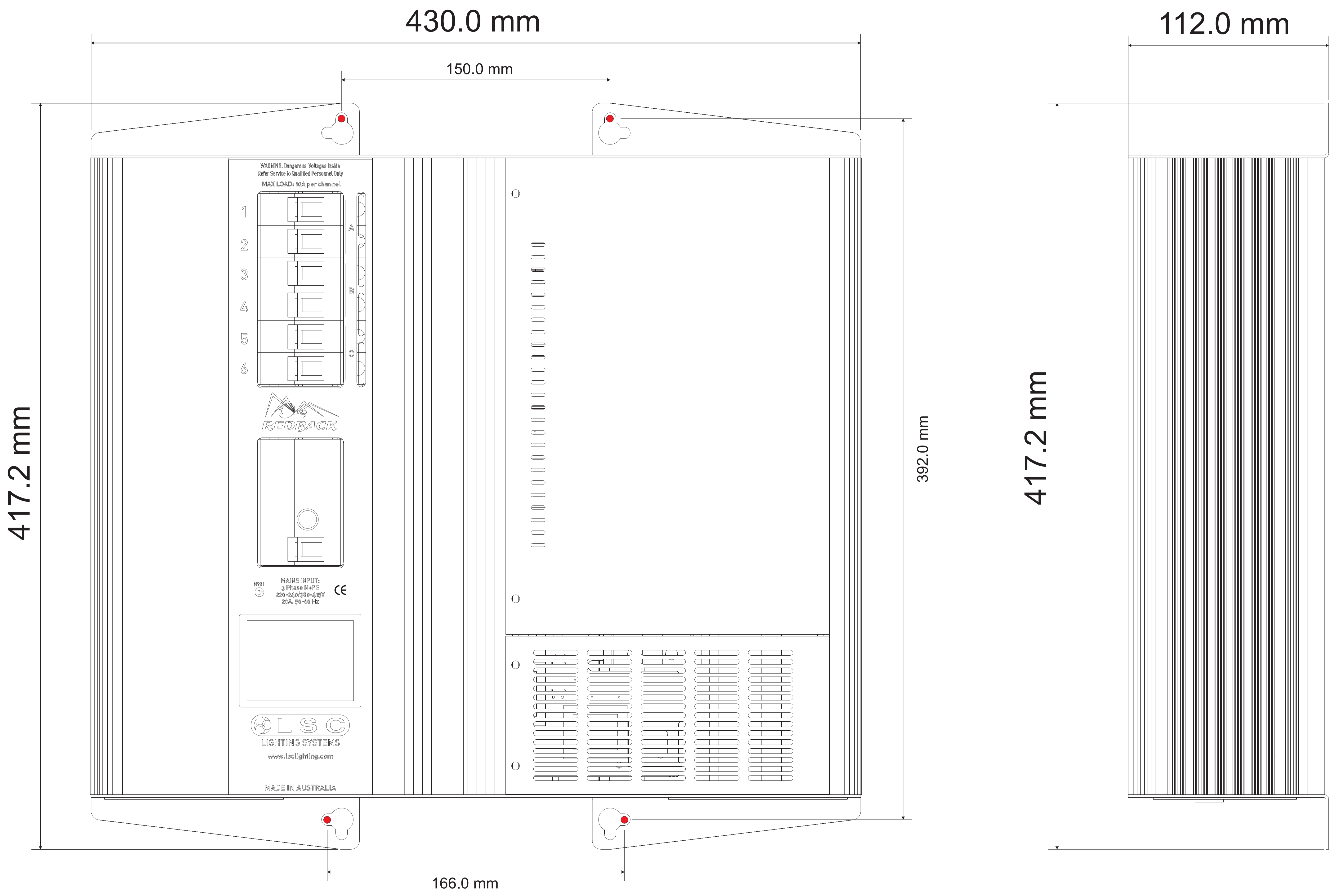
Redback 6 Channel Installation Dimmer Outline Drawing LSC Lighting systems
