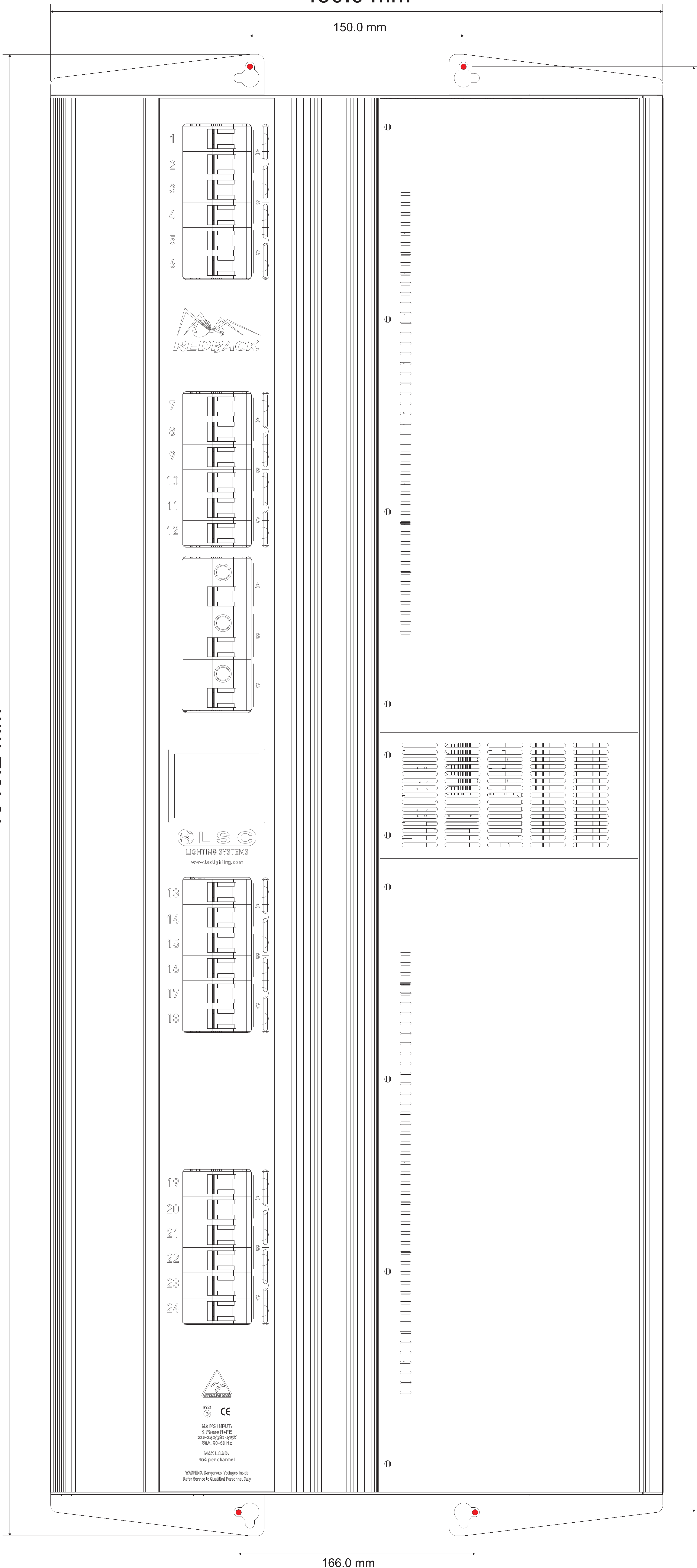
Redback 24 Channel Installation Dimmer Outline Drawing LSC Lighting systems
